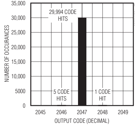
HISTOGRAM FOR 30,000 CONVERSIONS ( f_{\text{SAMPLE}} = 3.0\text{Msps} )
