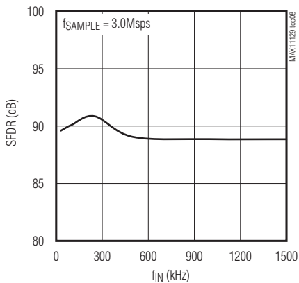
SFDR vs. ANALOG INPUT FREQUENCY
