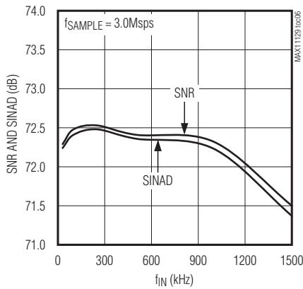
SNR AND SINAD vs. ANALOG INPUT FREQUENCY
